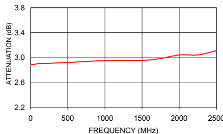
LAT-3+ ATTENUATION
