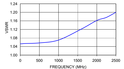
LAT-3+ VSWR
